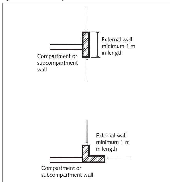
Figure 7 Junction of compartment walls and external walls
