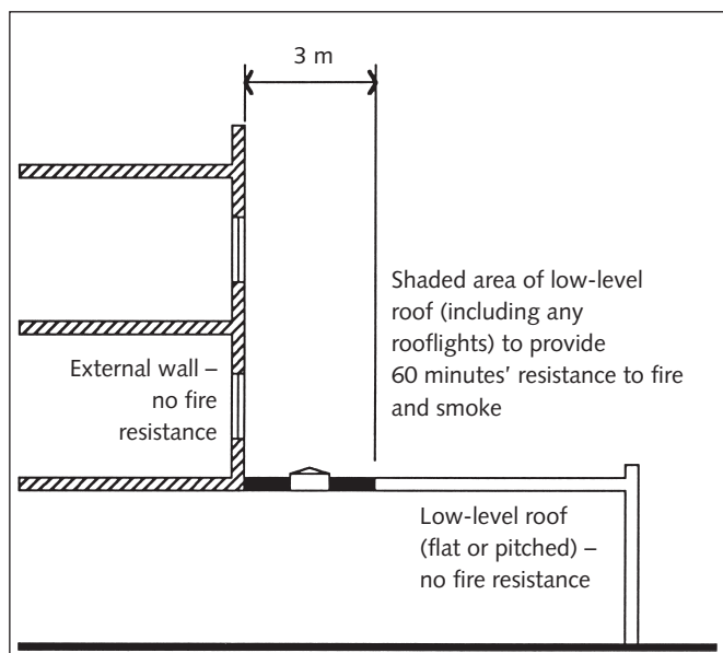
Figure 6 Fire resistance at junction of external walls and low-level roofs
