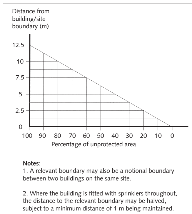
Figure 8 Unprotected areas
