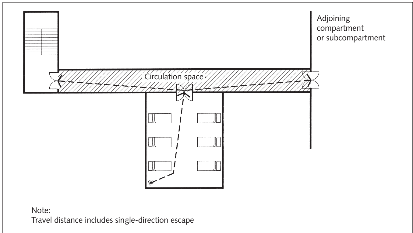
Figure 3 Measurement of overall escape distance
