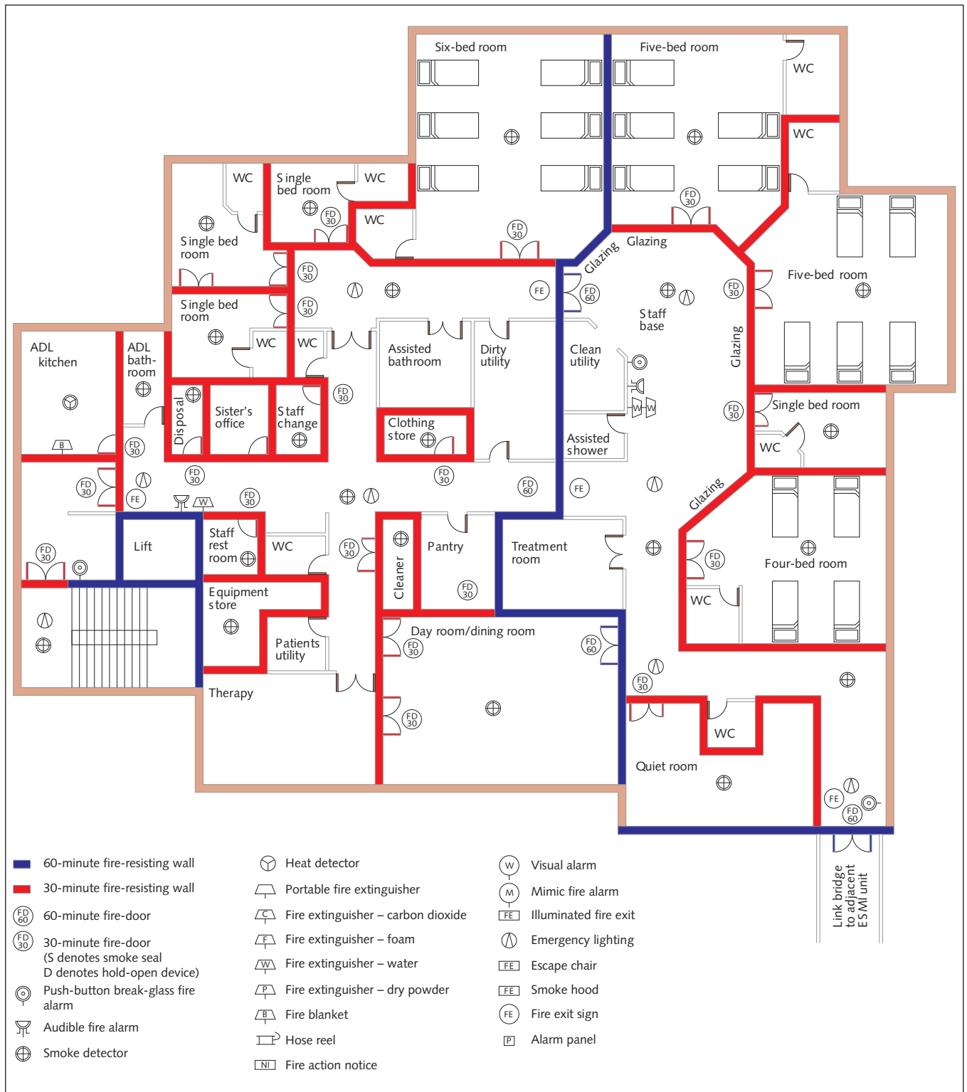
Figure 9 Example of a line drawing showing general fire safety precautions
